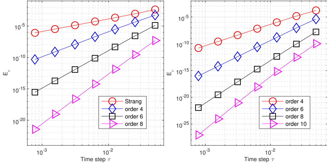
Figure 3: Successive errors E_\tau versus time step \tau for Eq. (28) of the composition methods starting from the Strang scheme (left) and the fourth order scheme S_\tau^{[4]} (right).
